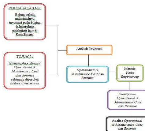
Figure.1. Research Flowchart
