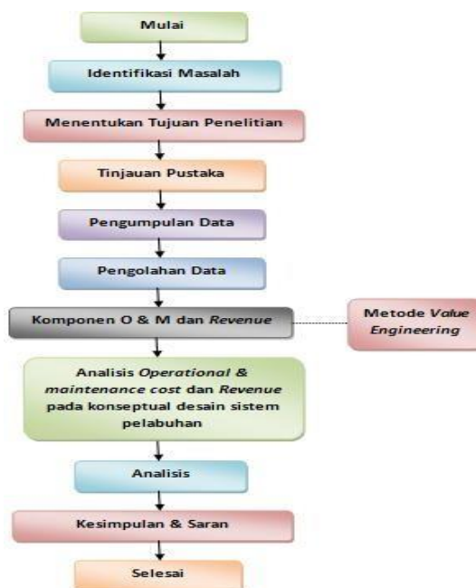
Figure.2. Research Framework
